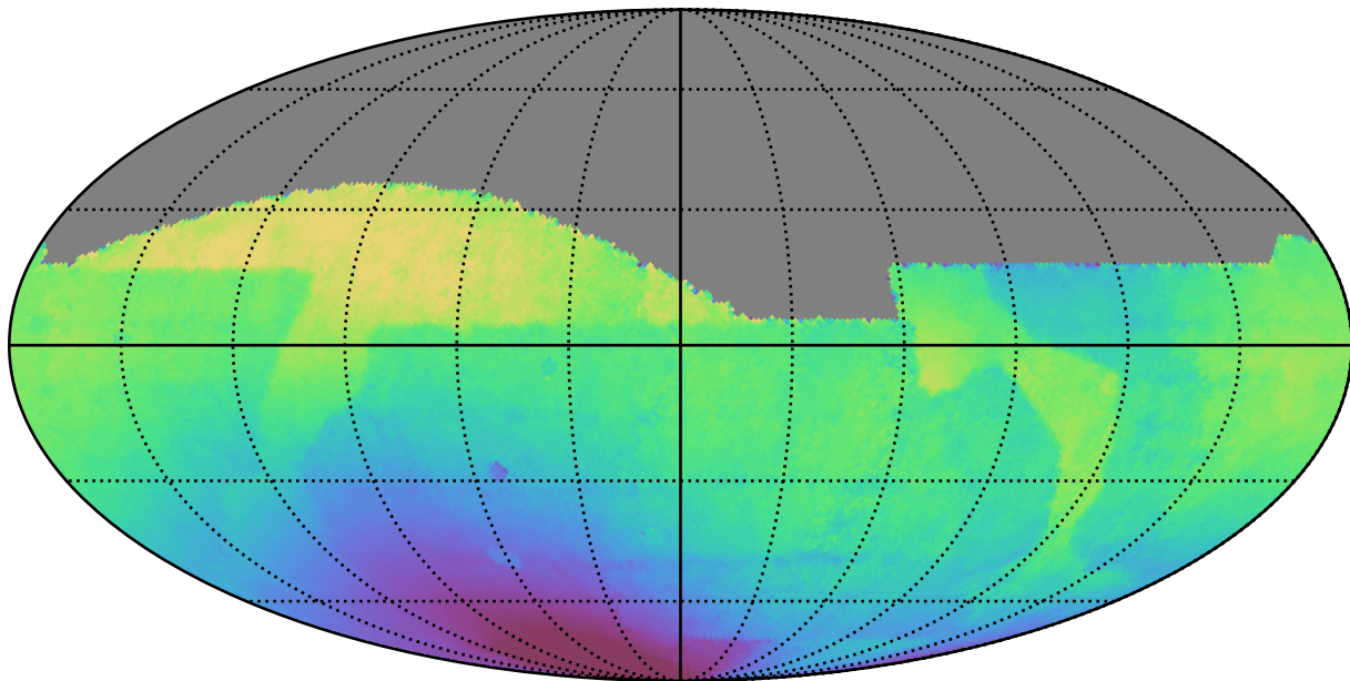
baseline_v2.1_10yrs All sky all bands: Median solarElong
