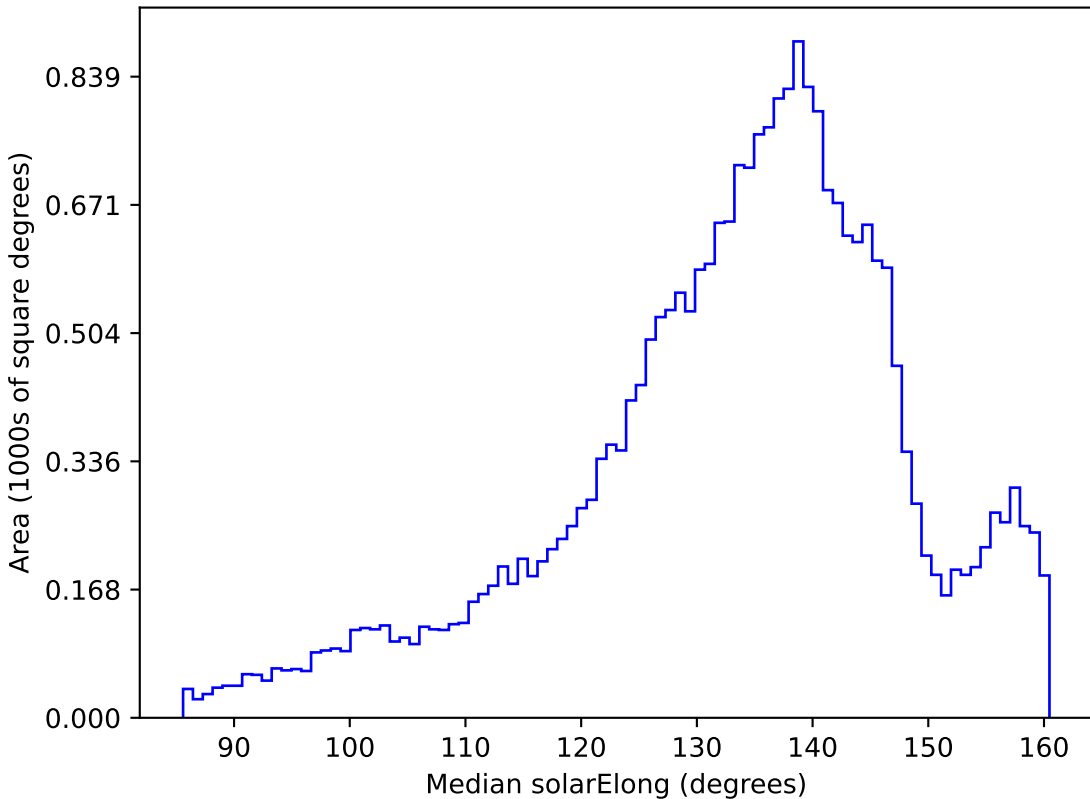
baseline_v2.1_10yrs All sky all bands: Median solarElong
