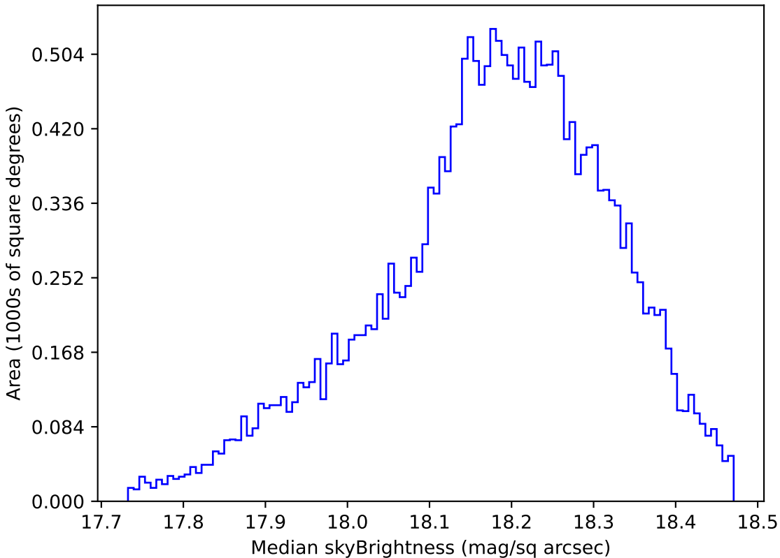
baseline_v2.1_10yrs Yr 1 y band: Median skyBrightness
