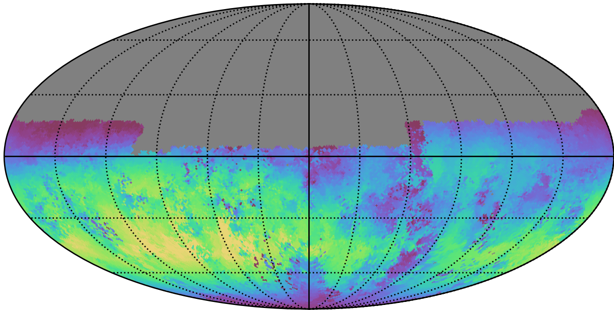
baseline_v2.1_10yrs Yr 1 u band: Median skyBrightness
