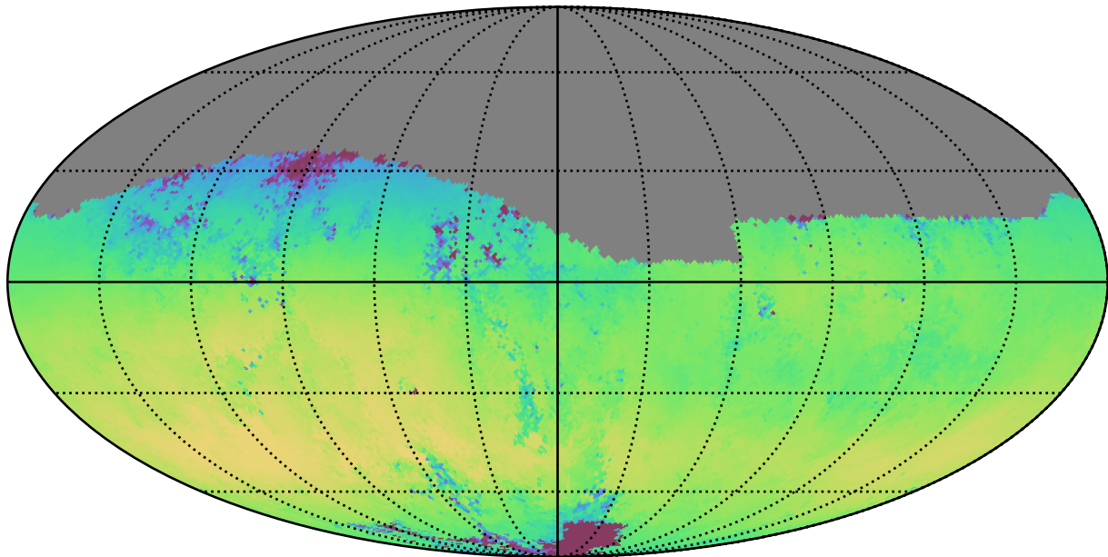
baseline_v2.1_10yrs Yr 1 r band: Median skyBrightness
