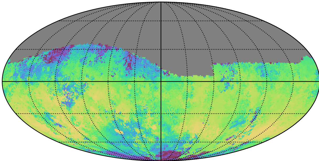
baseline_v2.1_10yrs Yr 1 i band: Median skyBrightness
