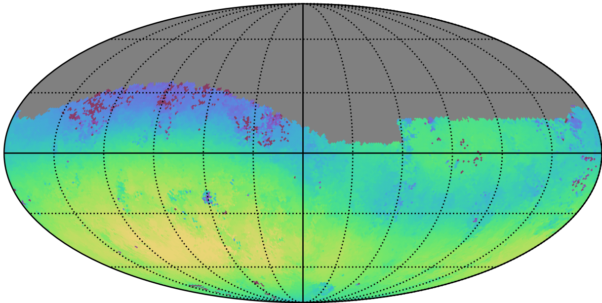
baseline_v2.1_10yrs Yr 1 g band: Median skyBrightness
