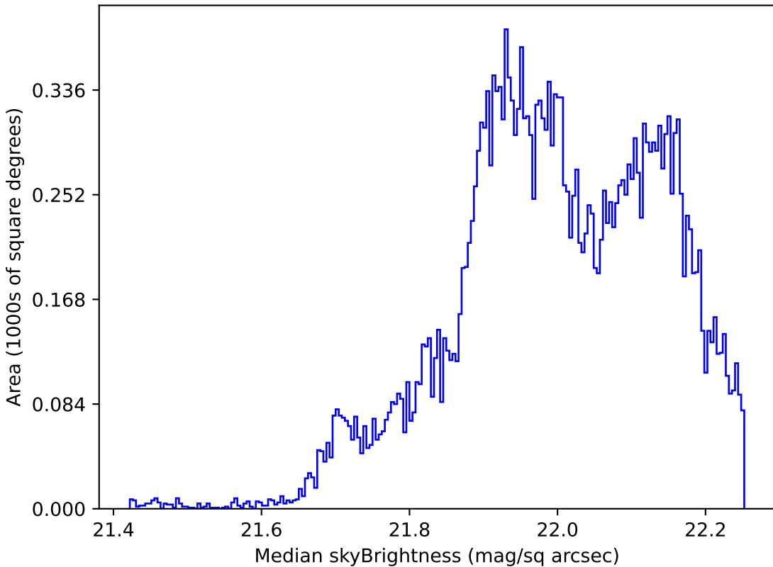
baseline_v2.1_10yrs Yr 1 g band: Median skyBrightness
