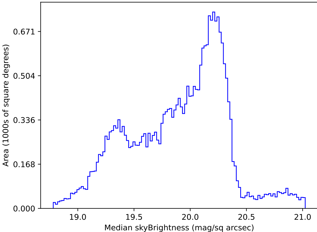
baseline_v2.1_10yrs Yr 1 all bands: Median skyBrightness
