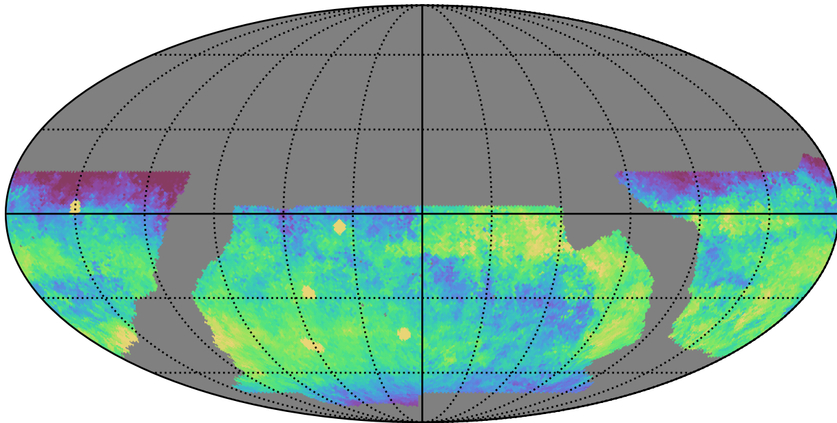
baseline_v2.1_10yrs WFD z band: Median skyBrightness
