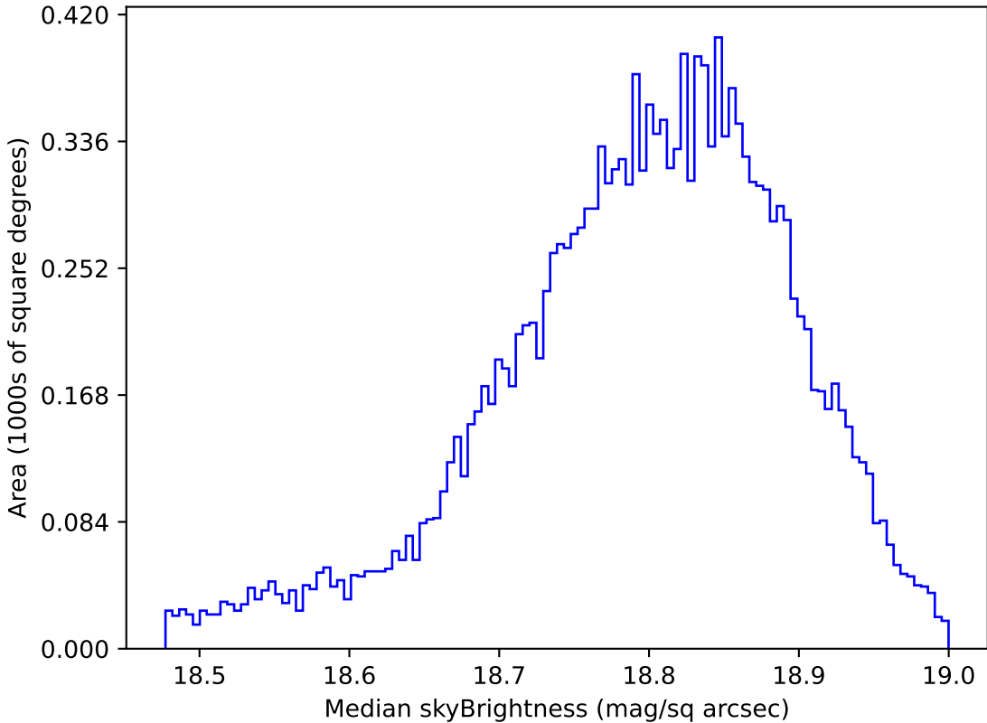
baseline_v2.1_10yrs WFD z band: Median skyBrightness
