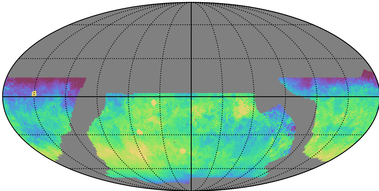
baseline_v2.1_10yrs WFD y band: Median skyBrightness
