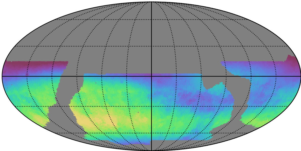
baseline_v2.1_10yrs WFD u band: Median skyBrightness
