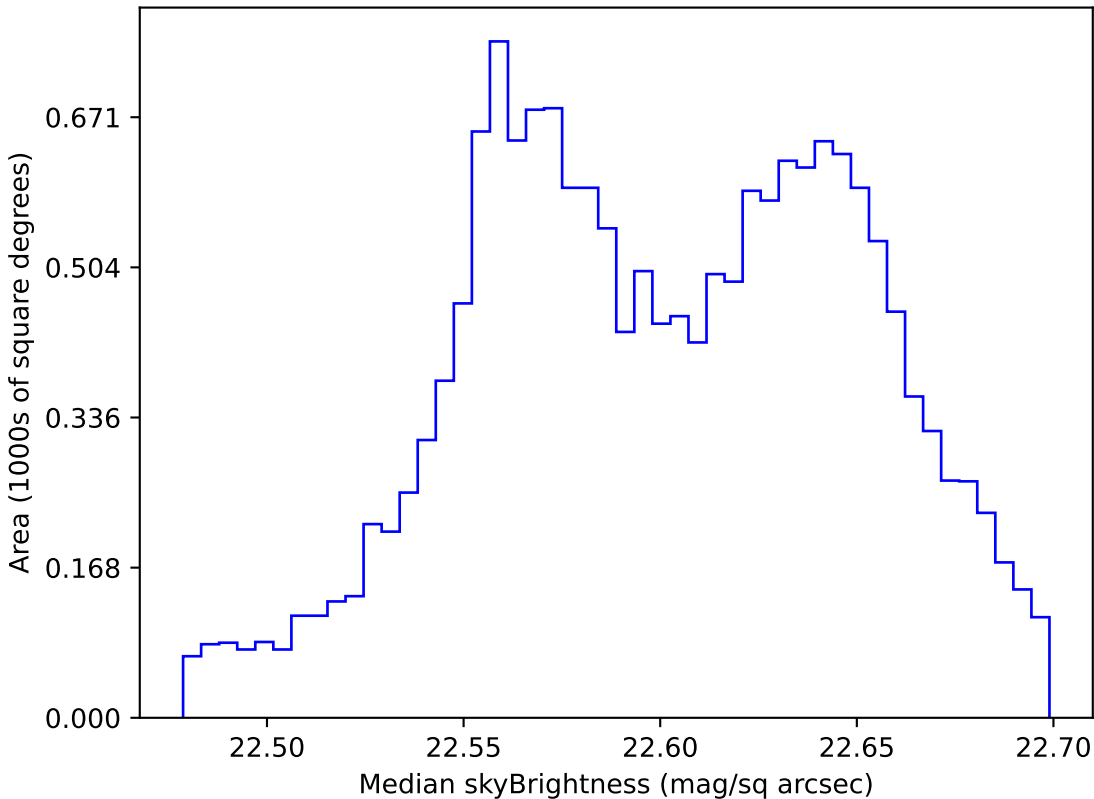
baseline_v2.1_10yrs WFD u band: Median skyBrightness
