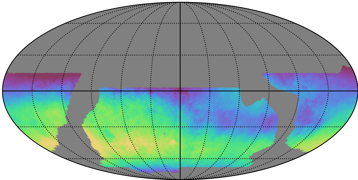
baseline_v2.1_10yrs WFD r band: Median skyBrightness
