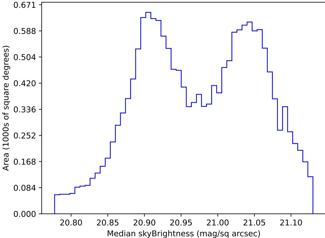
baseline_v2.1_10yrs WFD r band: Median skyBrightness
