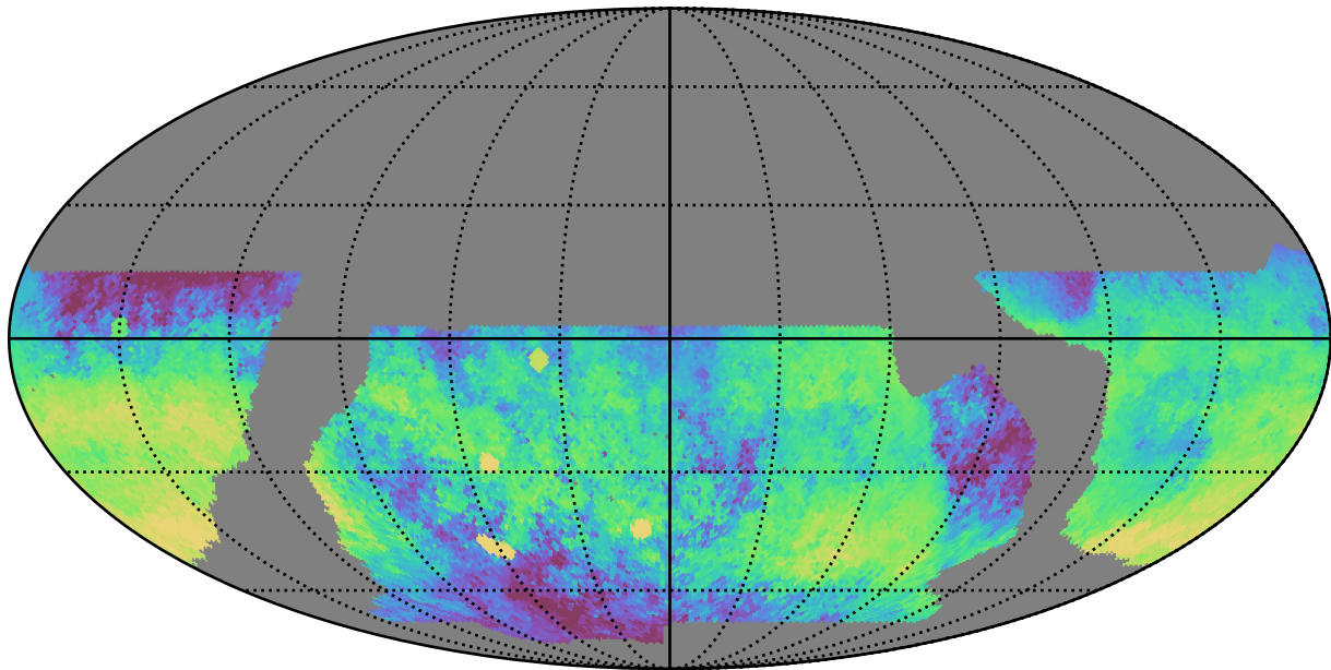
baseline_v2.1_10yrs WFD i band: Median skyBrightness
