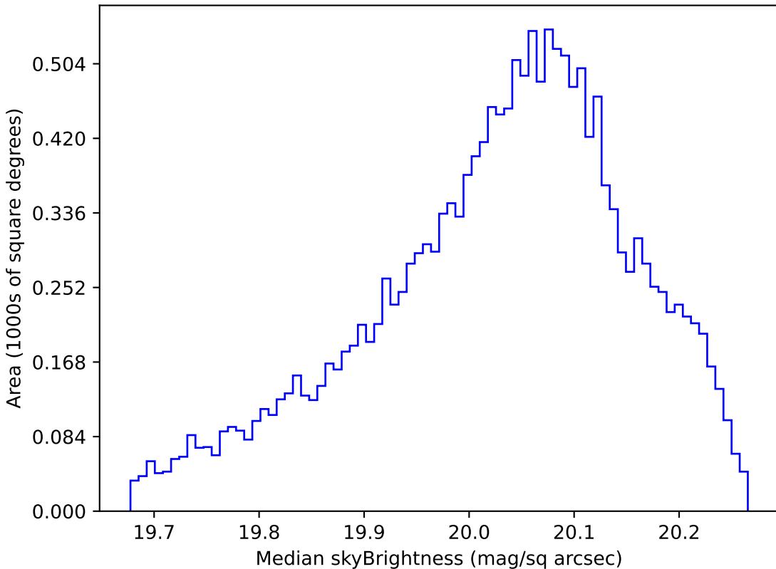
baseline_v2.1_10yrs WFD i band: Median skyBrightness
