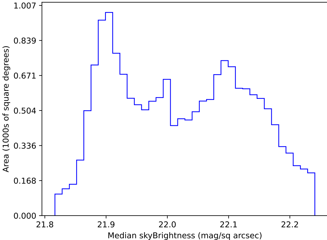
baseline_v2.1_10yrs WFD g band: Median skyBrightness
