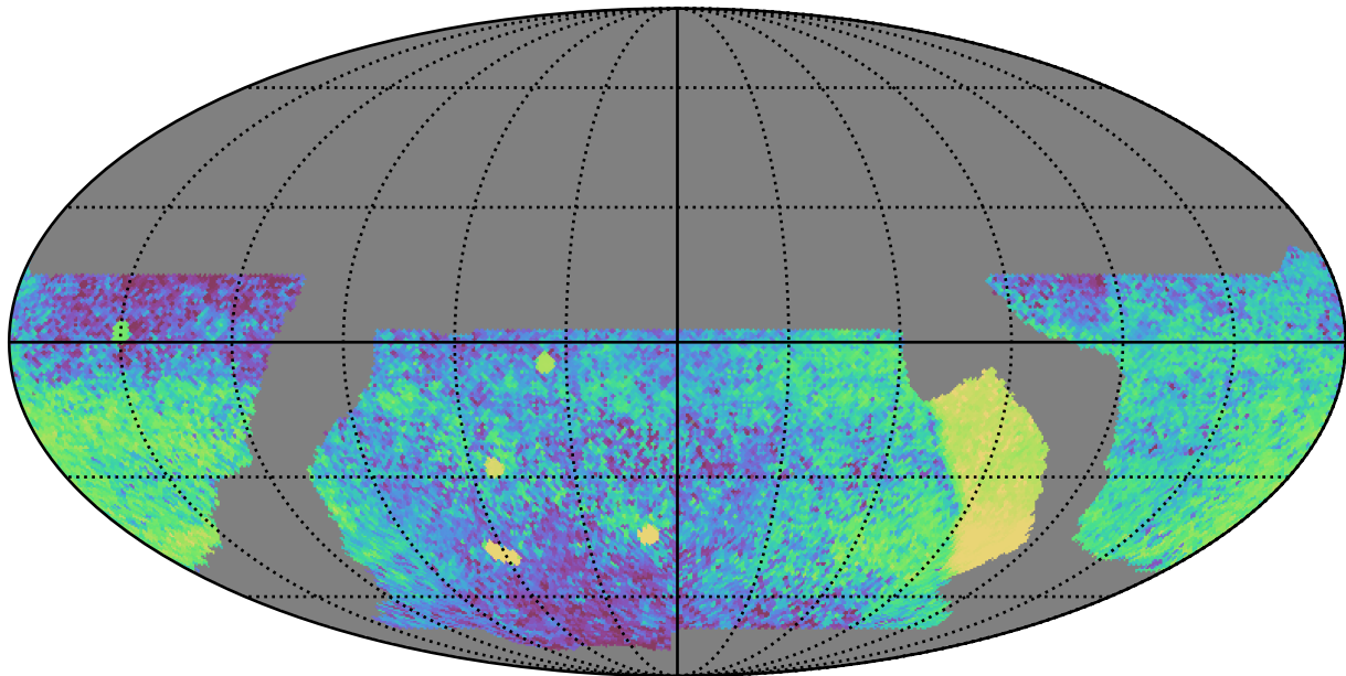
baseline_v2.1_10yrs WFD all bands: Median skyBrightness
