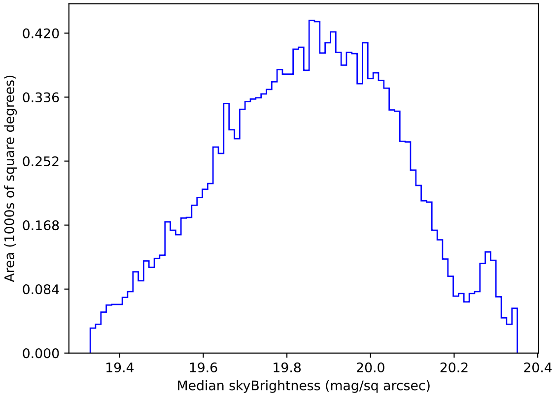
baseline_v2.1_10yrs WFD all bands: Median skyBrightness
