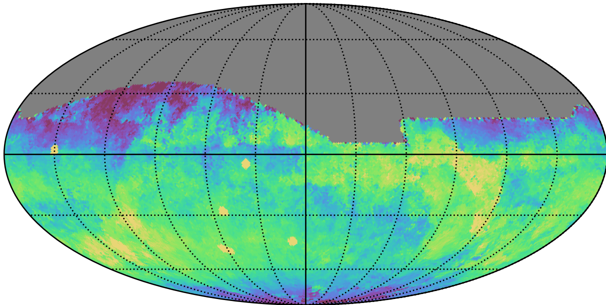
baseline_v2.1_10yrs All sky z band: Median skyBrightness
