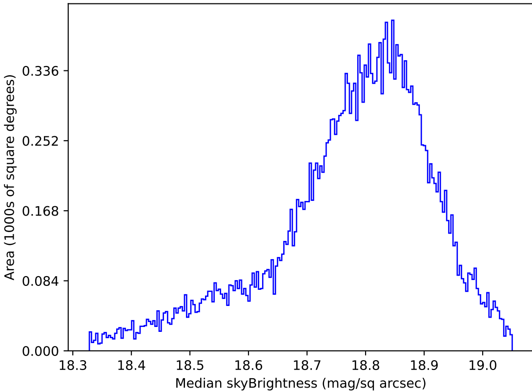
baseline_v2.1_10yrs All sky z band: Median skyBrightness
