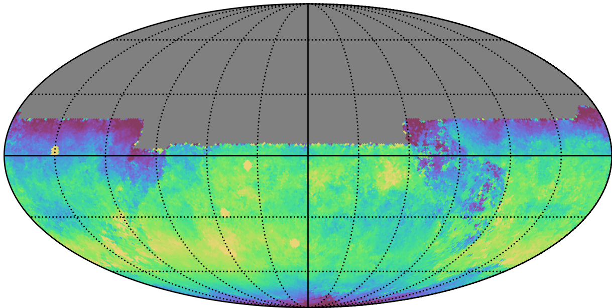
baseline_v2.1_10yrs All sky y band: Median skyBrightness
