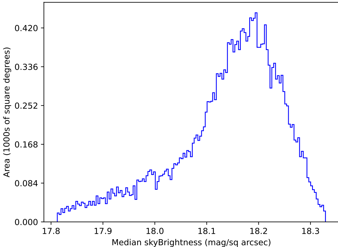
baseline_v2.1_10yrs All sky y band: Median skyBrightness
