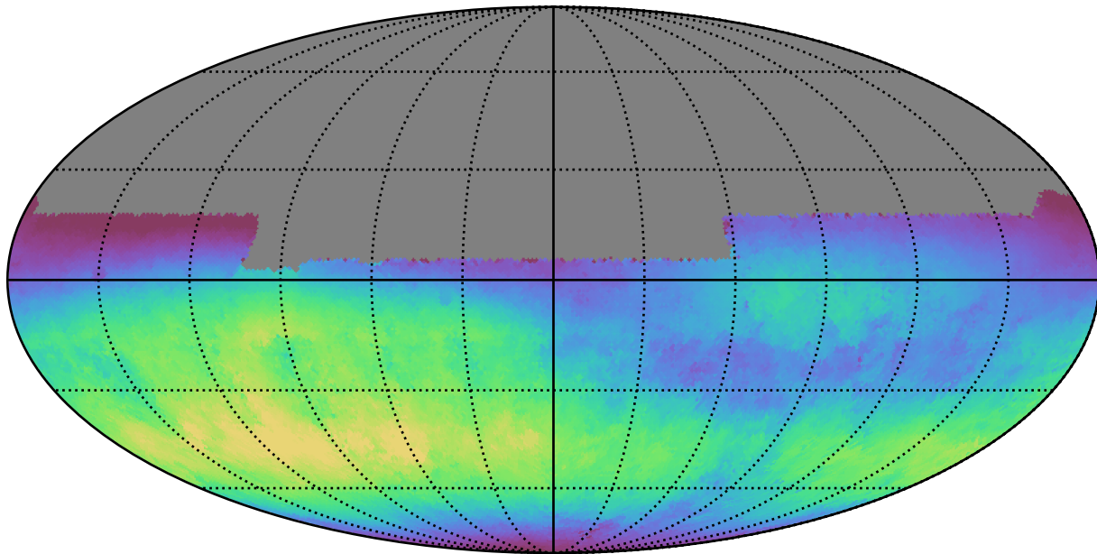
baseline_v2.1_10yrs All sky u band: Median skyBrightness
