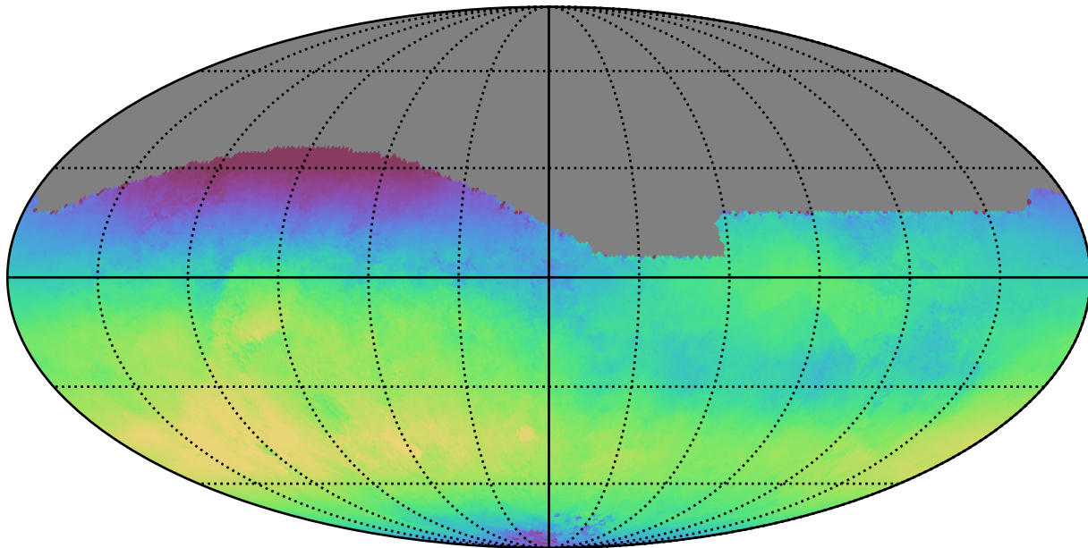
baseline_v2.1_10yrs All sky r band: Median skyBrightness
