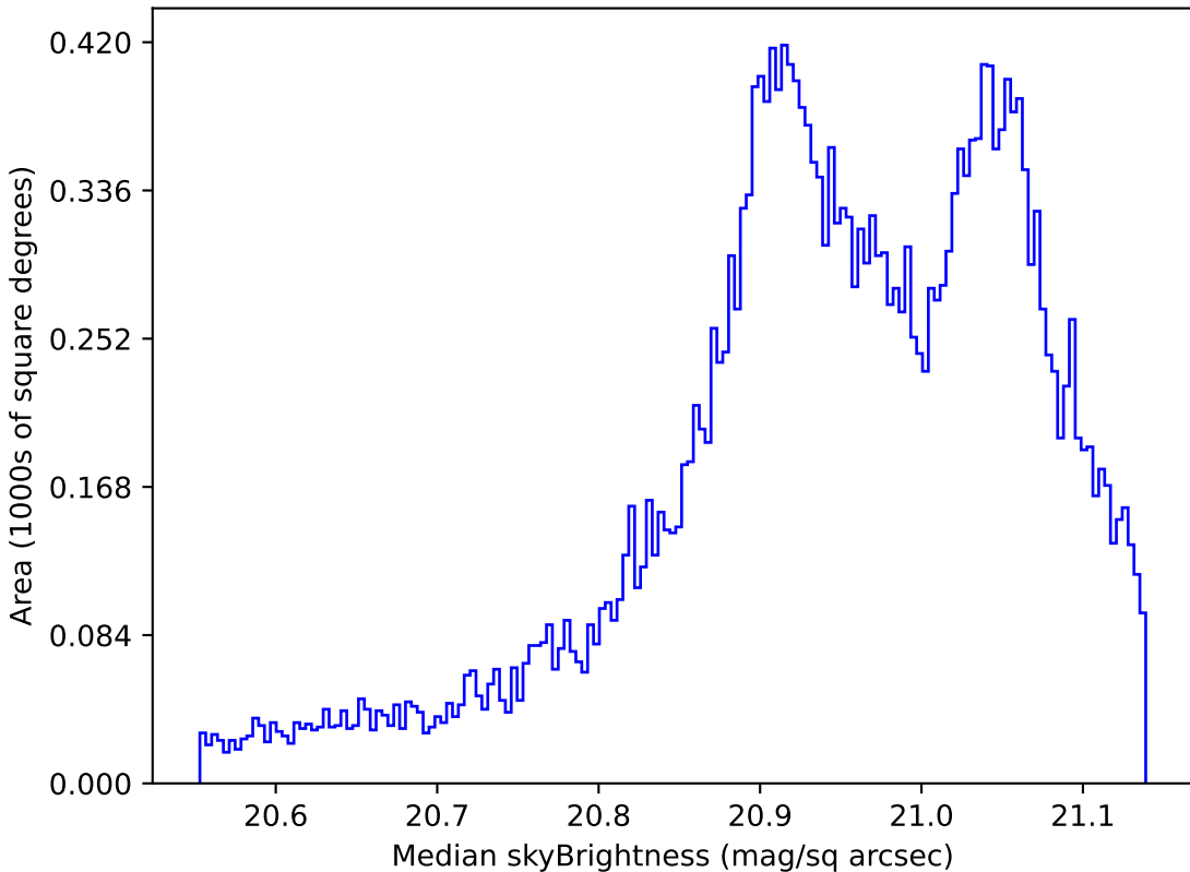
baseline_v2.1_10yrs All sky r band: Median skyBrightness
