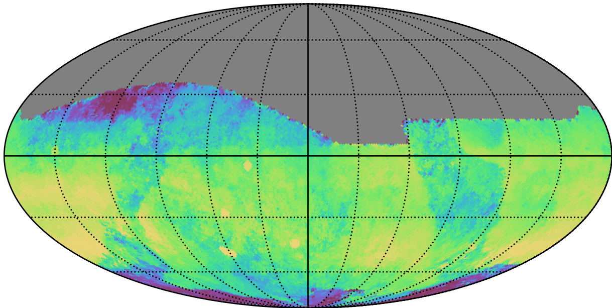
baseline_v2.1_10yrs All sky i band: Median skyBrightness
