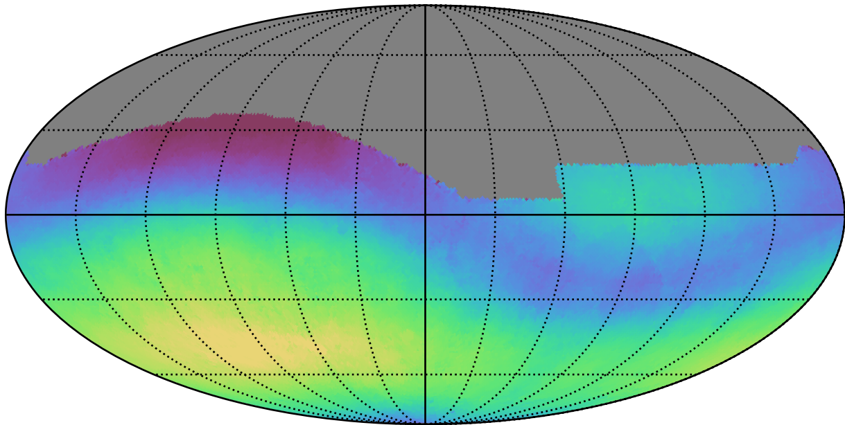
baseline_v2.1_10yrs All sky g band: Median skyBrightness
