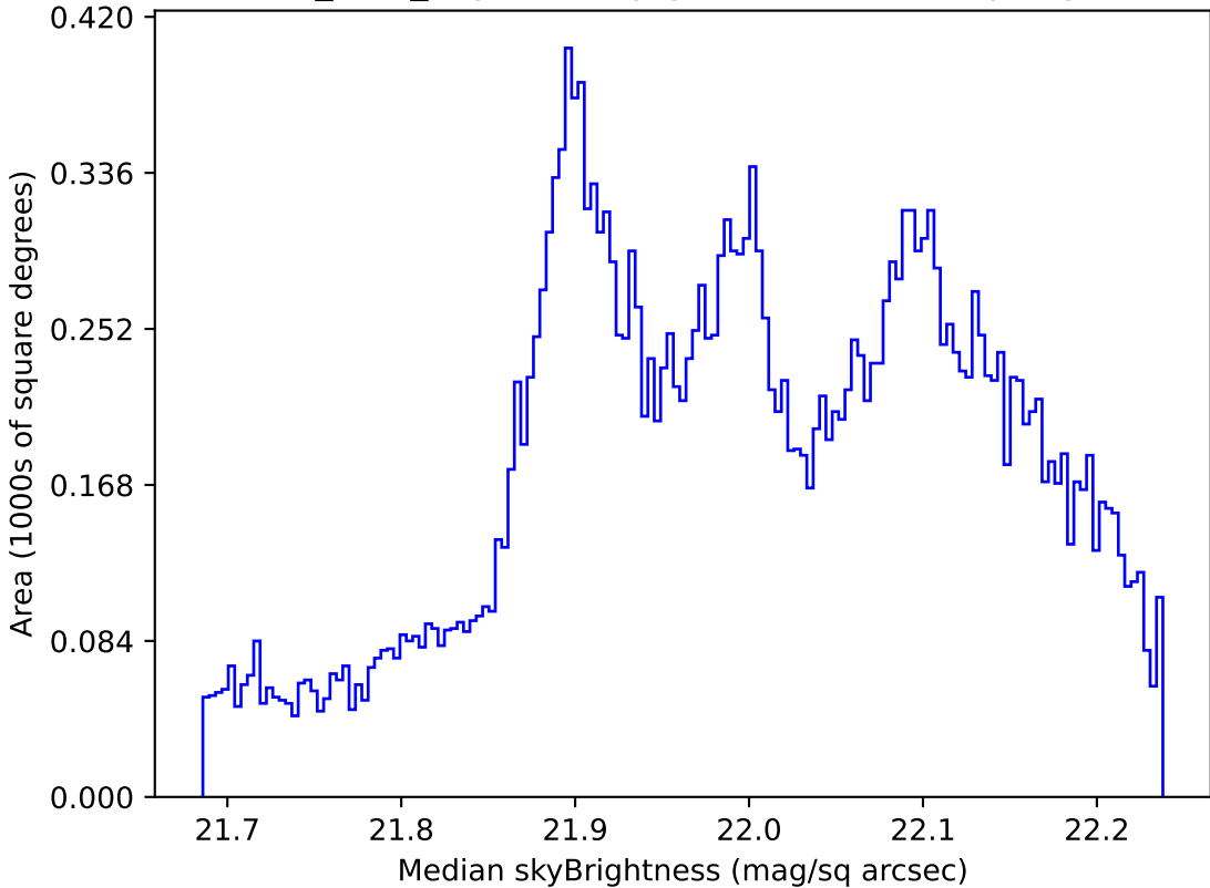
baseline_v2.1_10yrs All sky g band: Median skyBrightness
