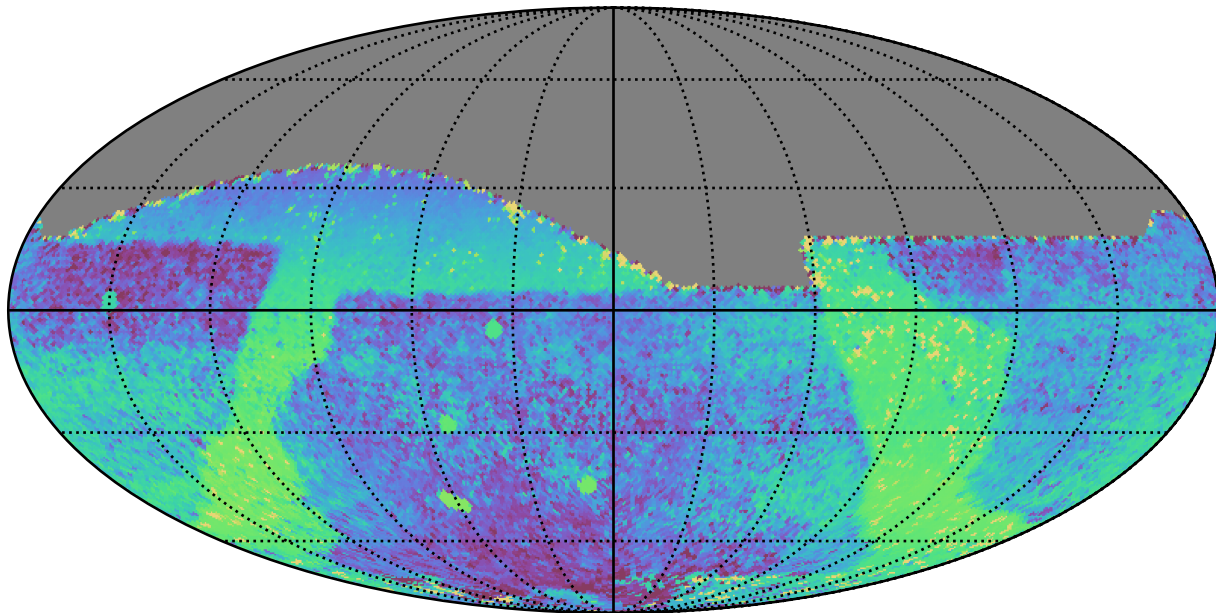
baseline_v2.1_10yrs All sky all bands: Median skyBrightness
