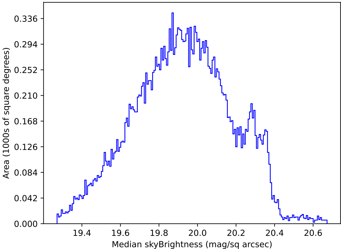
baseline_v2.1_10yrs All sky all bands: Median skyBrightness
