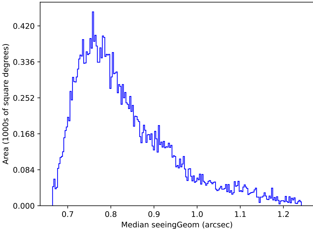
baseline_v2.1_10yrs Yr 1 z band: Median seeingGeom
