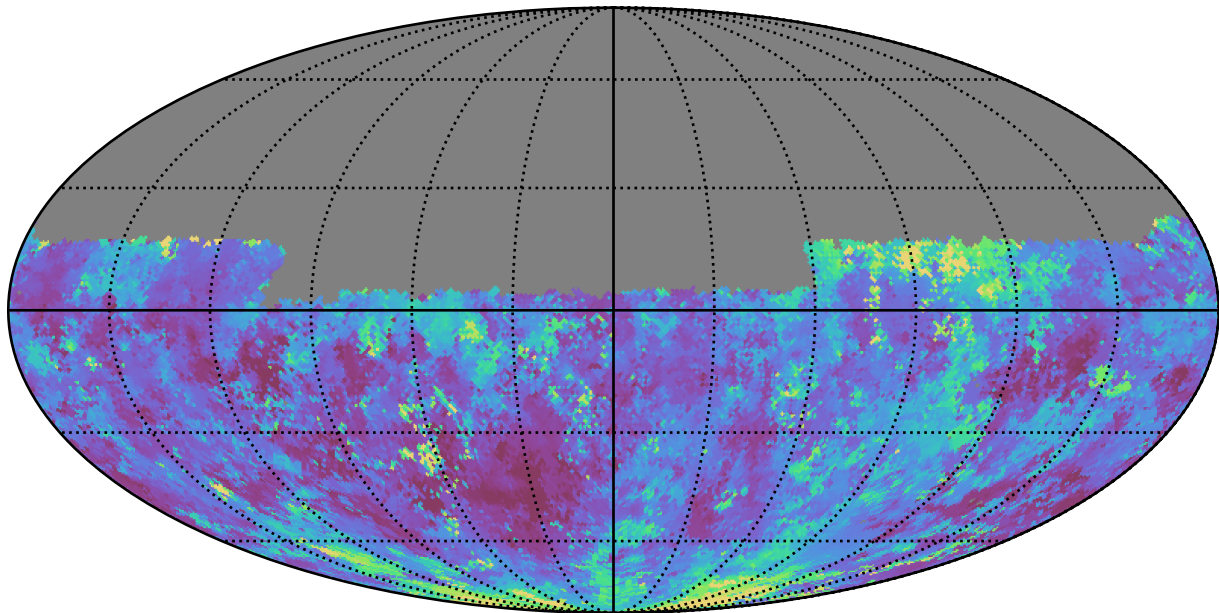
baseline_v2.1_10yrs Yr 1 u band: Median seeingGeom
