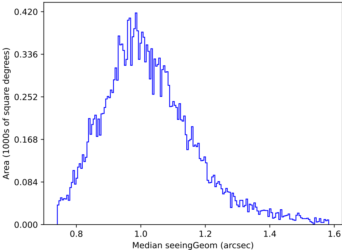
baseline_v2.1_10yrs Yr 1 u band: Median seeingGeom
