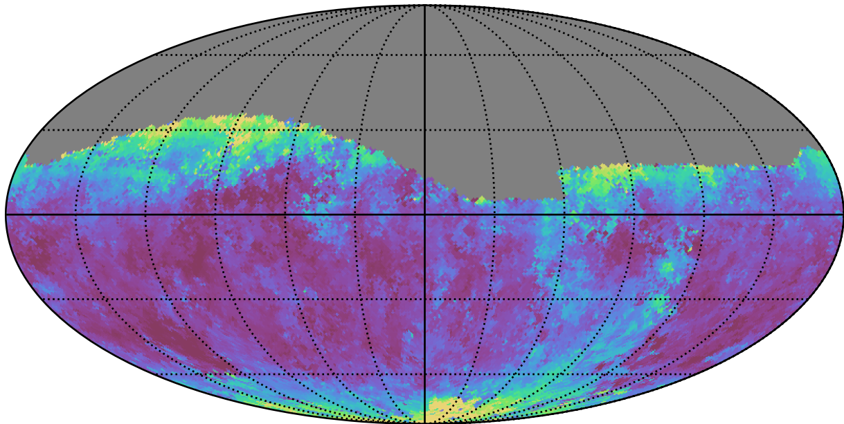
baseline_v2.1_10yrs Yr 1 r band: Median seeingGeom
