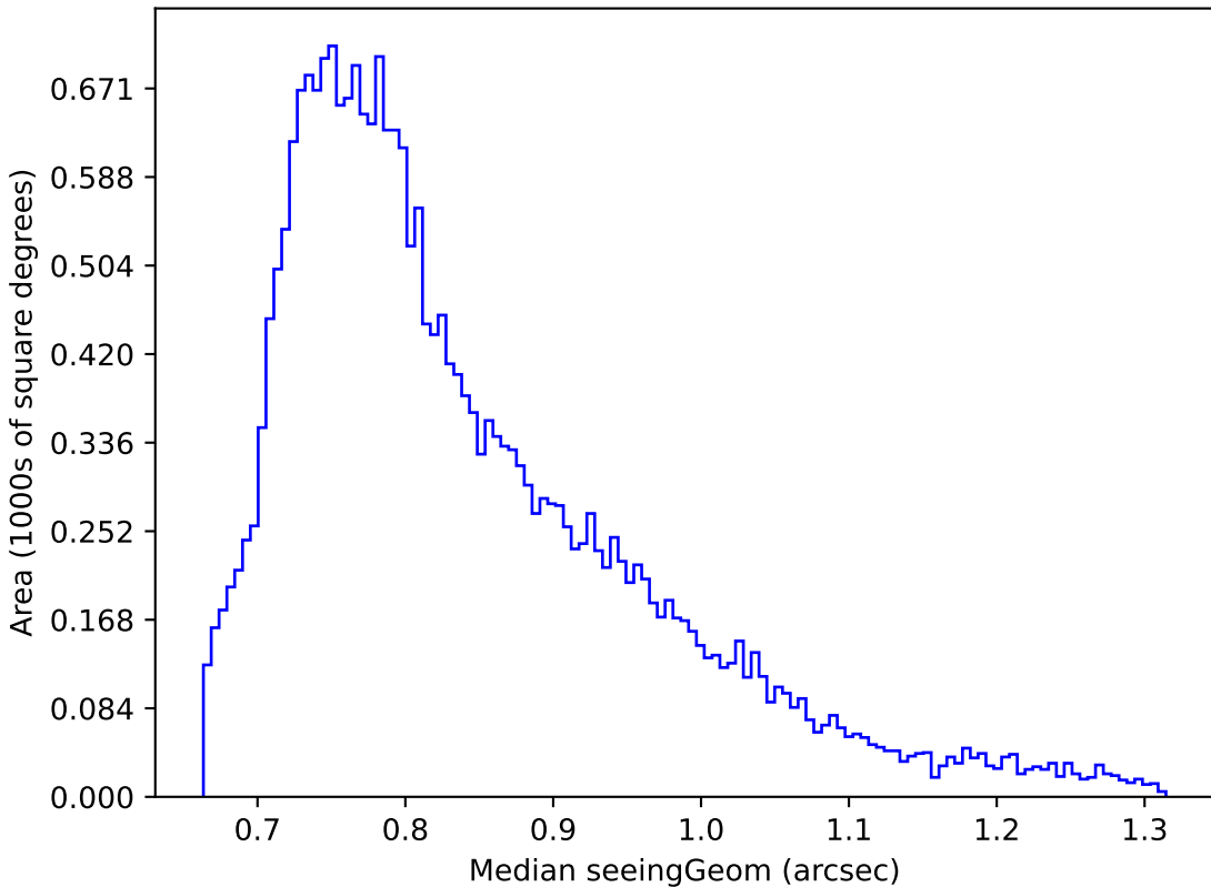
baseline_v2.1_10yrs Yr 1 r band: Median seeingGeom
