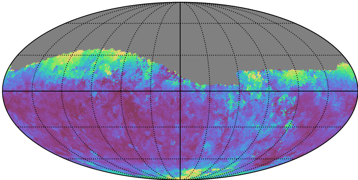
baseline_v2.1_10yrs Yr 1 i band: Median seeingGeom
