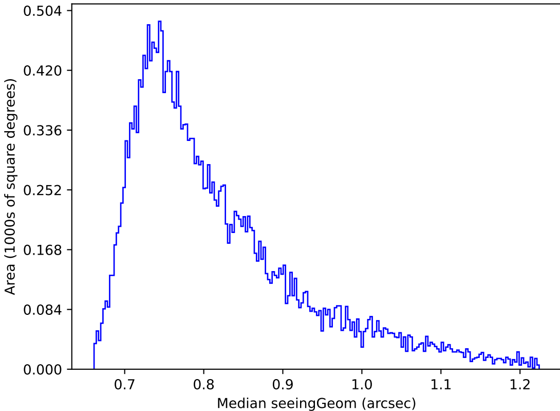
baseline_v2.1_10yrs Yr 1 i band: Median seeingGeom
