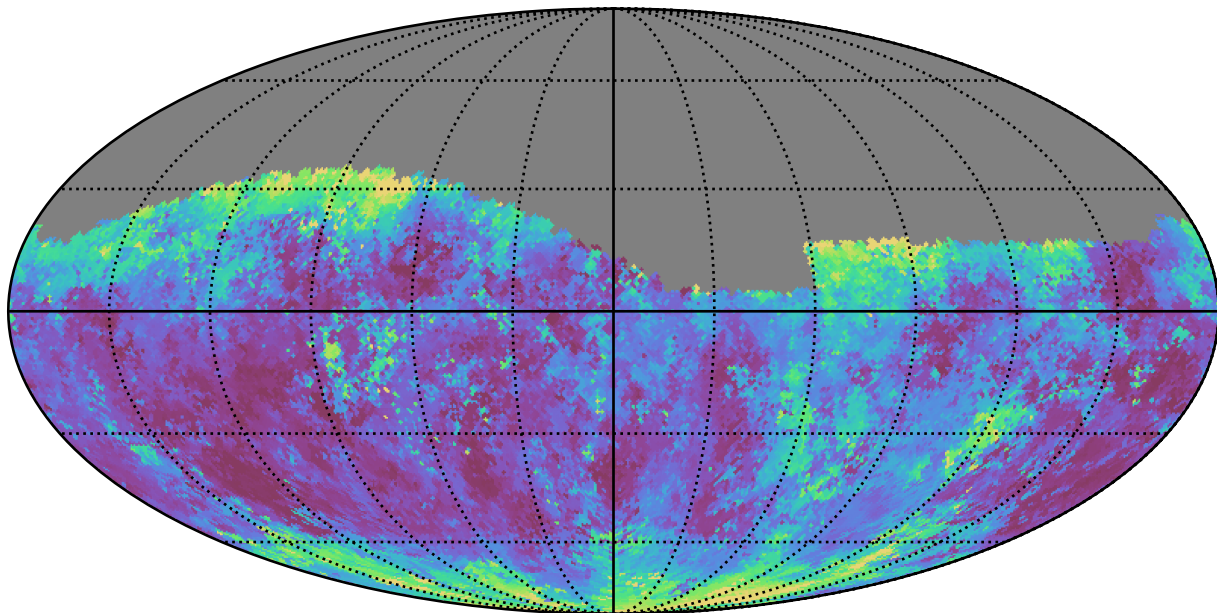
baseline_v2.1_10yrs Yr 1 g band: Median seeingGeom
