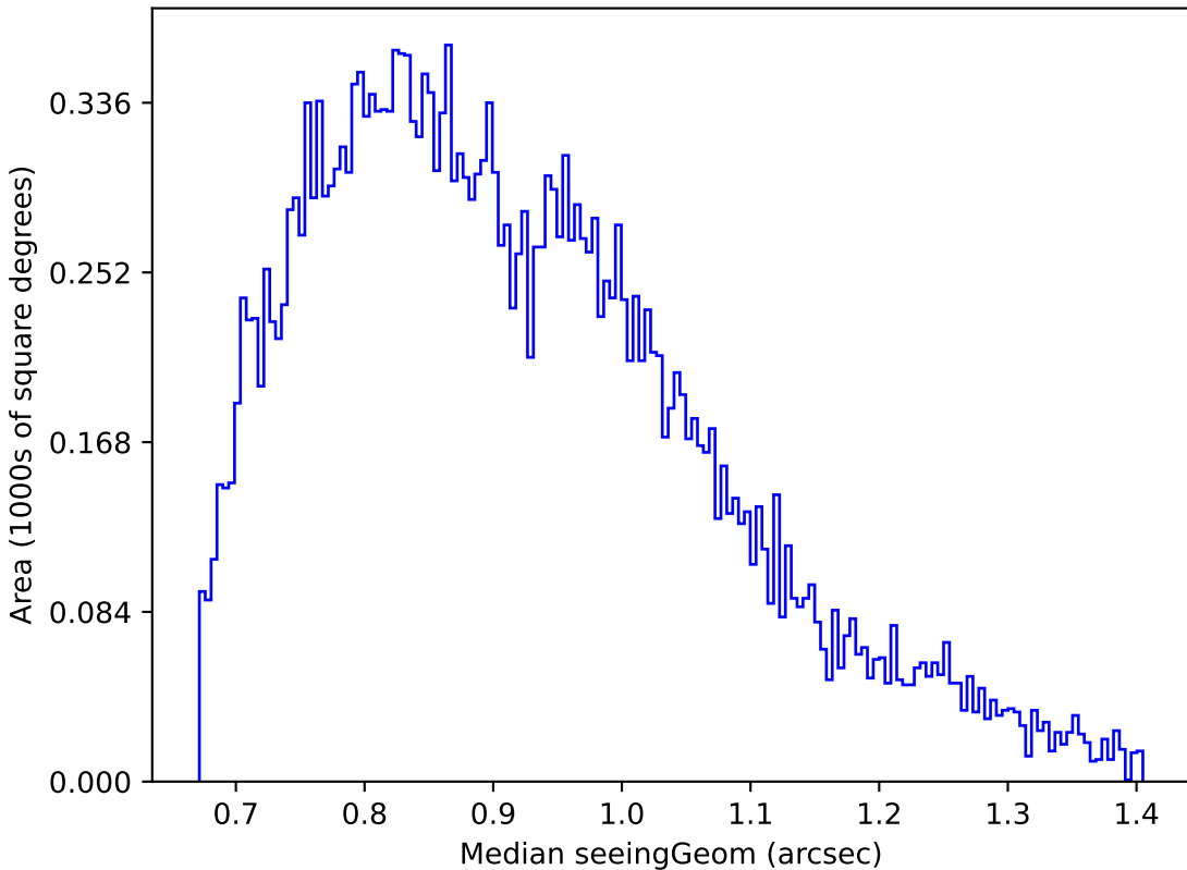
baseline_v2.1_10yrs Yr 1 g band: Median seeingGeom
