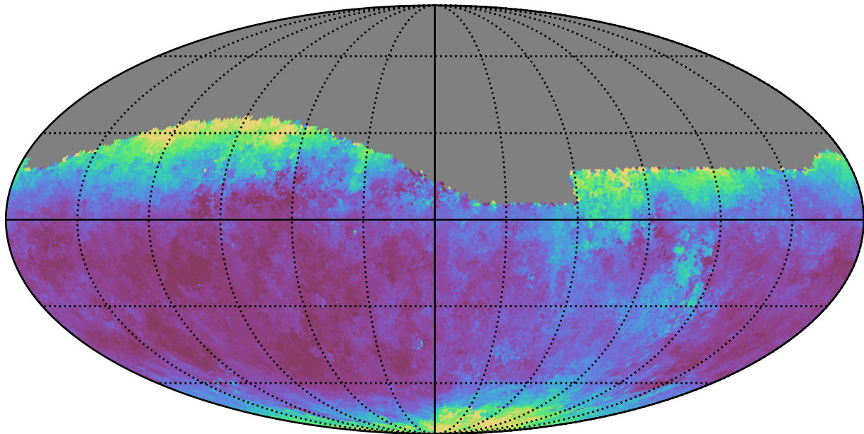
baseline_v2.1_10yrs Yr 1 all bands: Median seeingGeom
