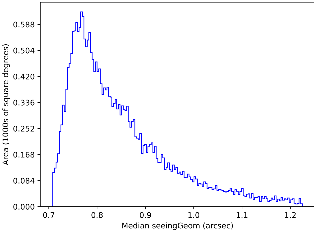
baseline_v2.1_10yrs Yr 1 all bands: Median seeingGeom
