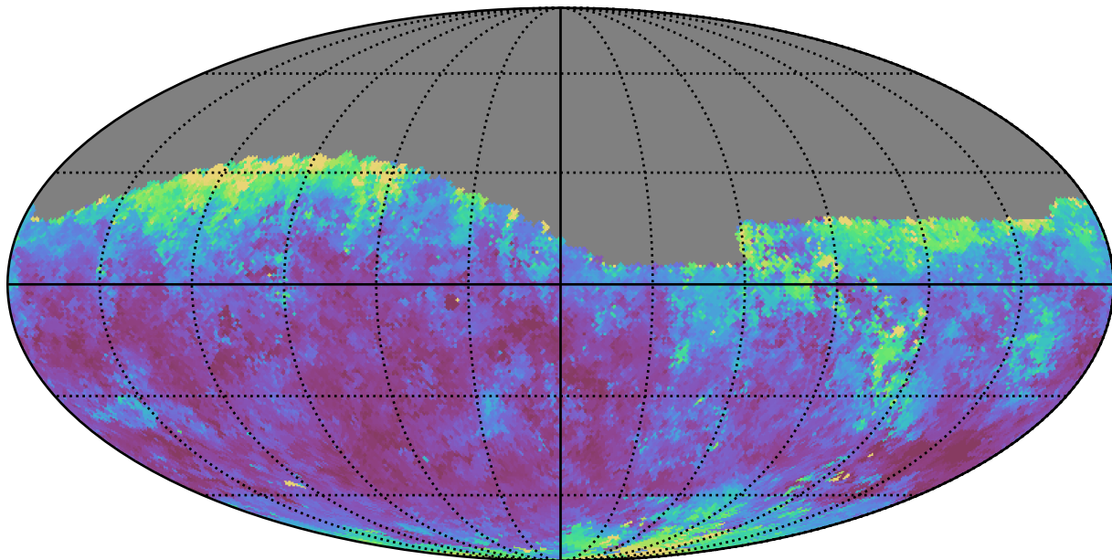
baseline_v2.1_10yrs Yr 1 z band: Median seeingEff
