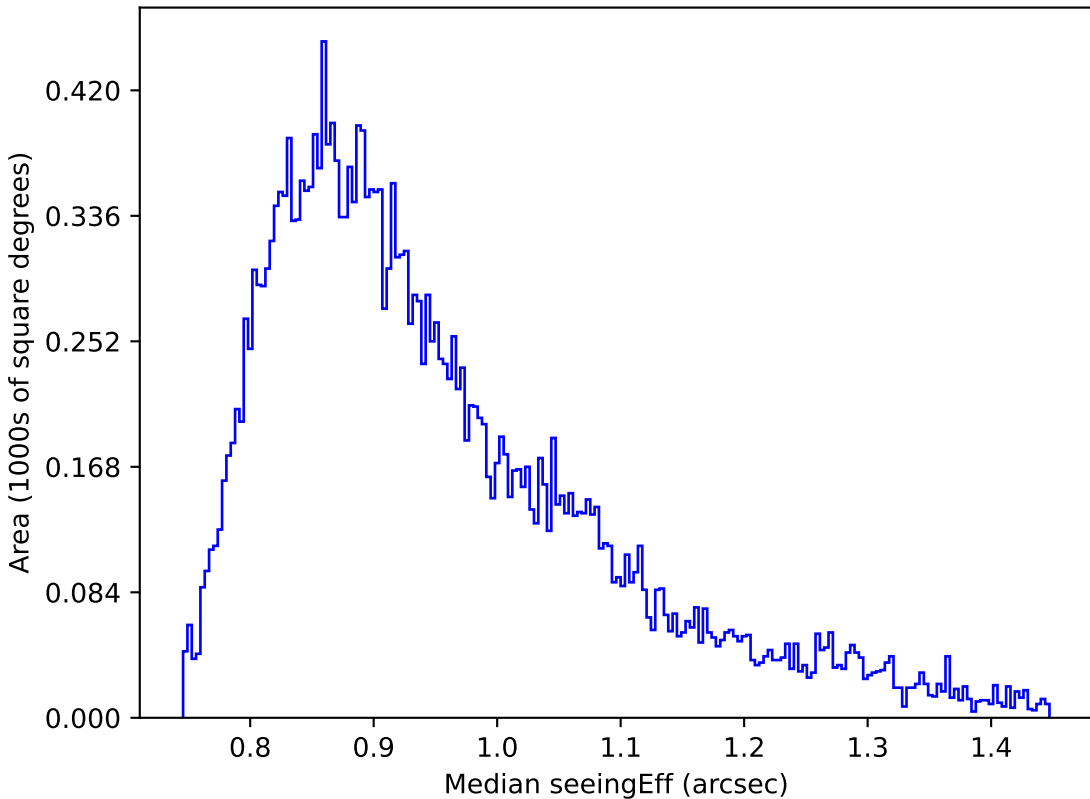
baseline_v2.1_10yrs Yr 1 z band: Median seeingEff
