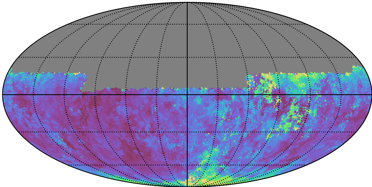
baseline_v2.1_10yrs Yr 1 y band: Median seeingEff
