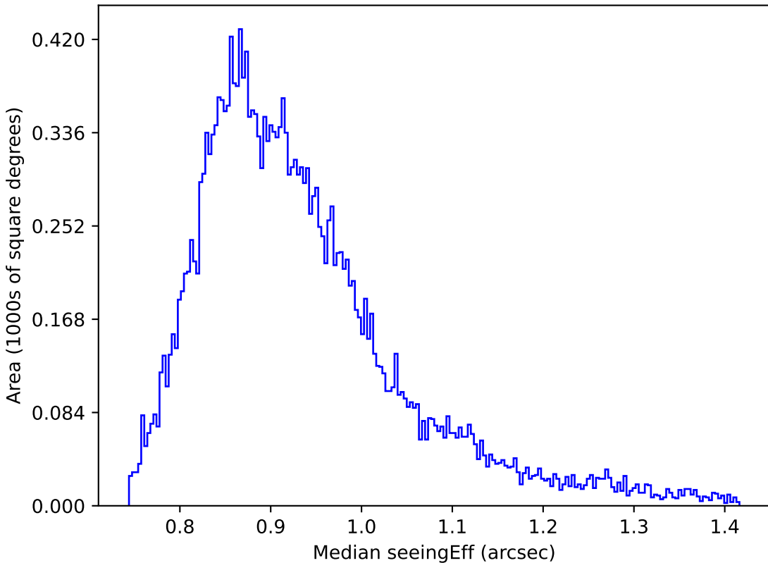
baseline_v2.1_10yrs Yr 1 y band: Median seeingEff
