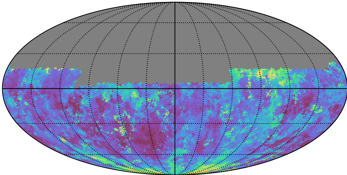
baseline_v2.1_10yrs Yr 1 u band: Median seeingEff
