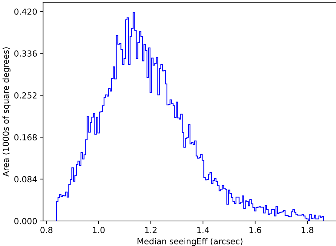
baseline_v2.1_10yrs Yr 1 u band: Median seeingEff
